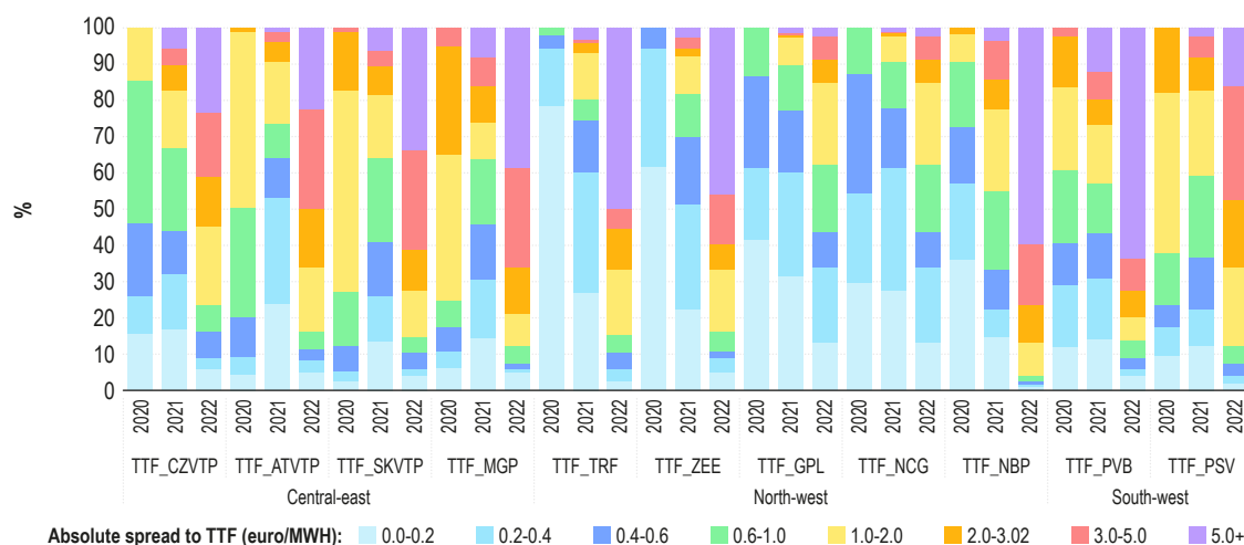
Figure 10: Day-ahead price convergence between TTF and selected EU hubs – 2020 – June 2022 – % of trading days within given price spread range
