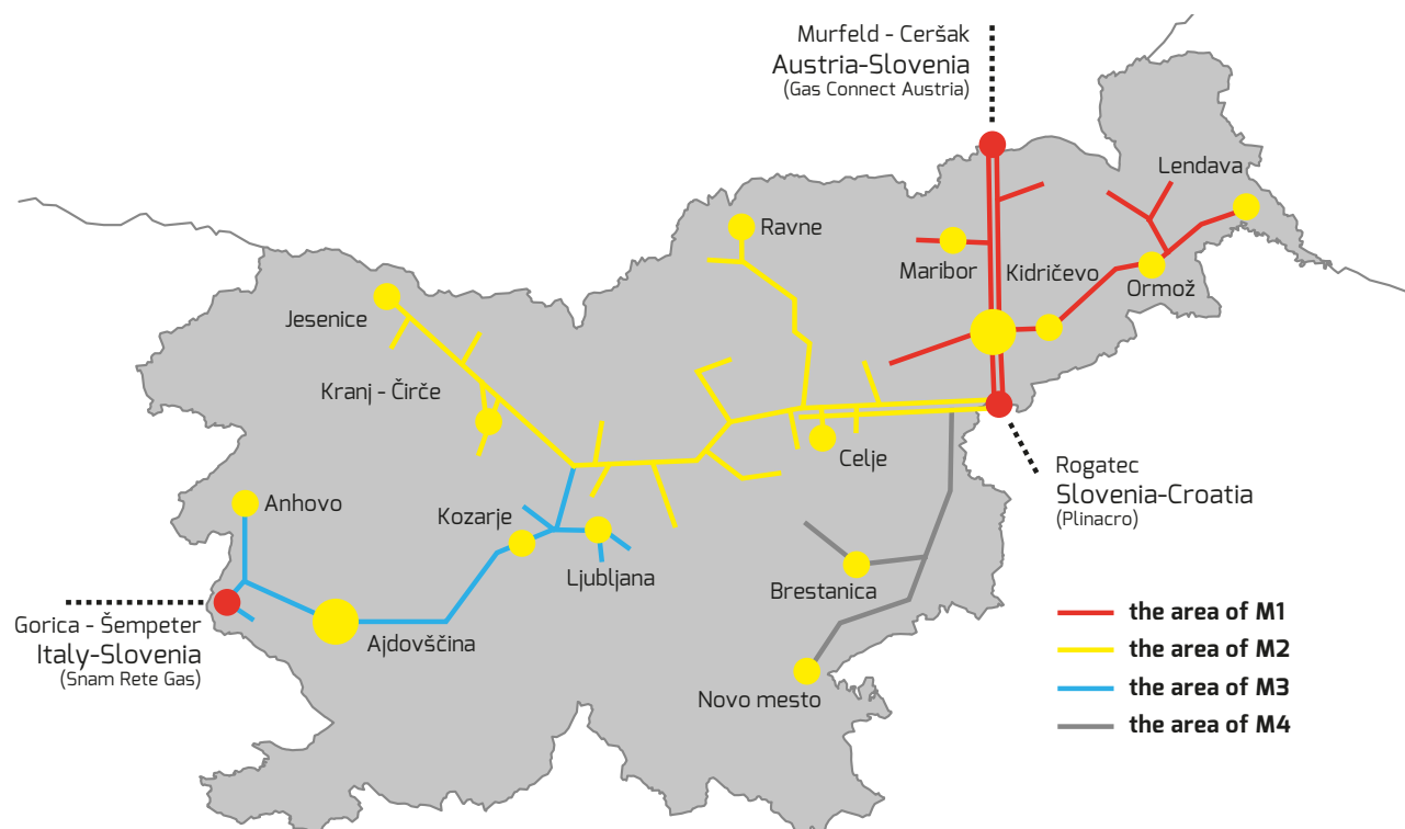
Figure 53: Schematic map of the gas network with relevant points
