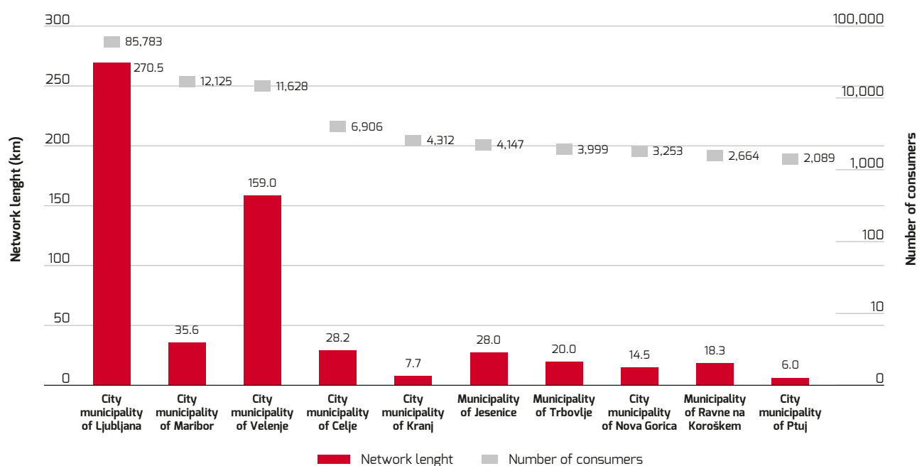
Figure 84: Length of heat distribution networks by municipality, and the numbers of connected users in 2013
