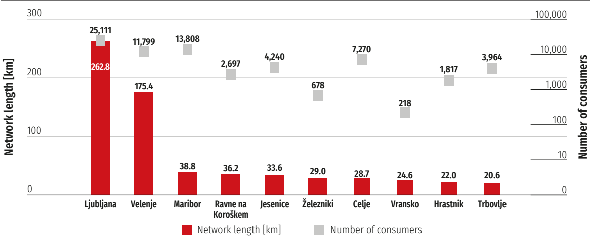
Figure 139 LENGTH OF HEAT DISTRIBUTION SYSTEMS BY MUNICIPALITY, AND NUMBERS OF CONNECTED USERS IN 2016
